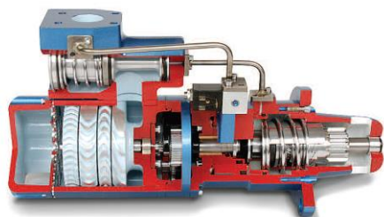
Pneumatic Starters
